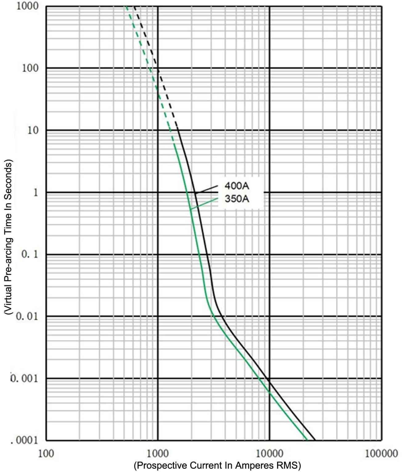
(Time-Current Characteristics Curve)
